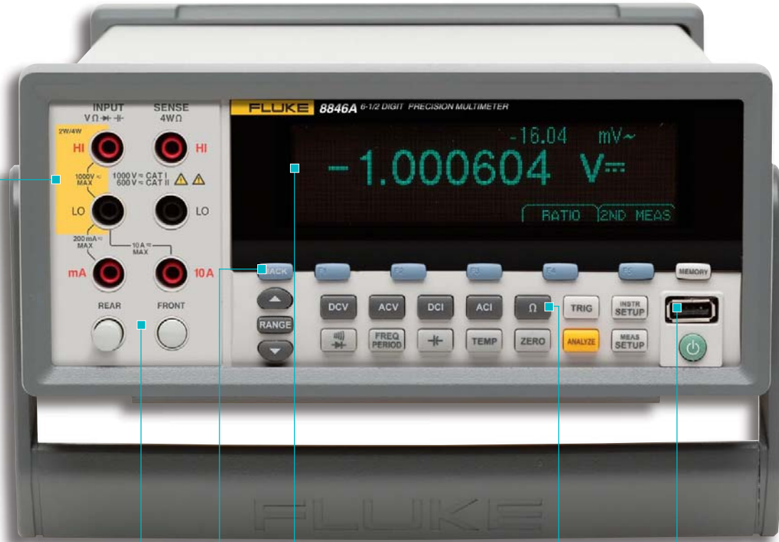
Patented split terminal jacks enable 4-wire measurements with two leads
